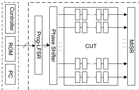
Fig. 1. Basic STUMPS Architecture.
