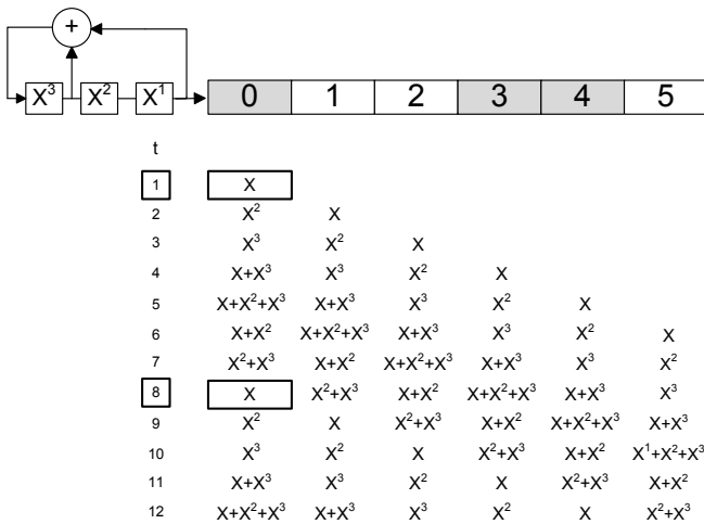
Fig. 5. LFSR sequence.
