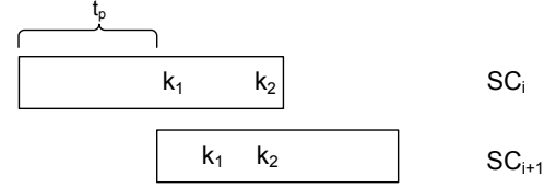
Fig. 4. Scan chain separation with and without conflict.
