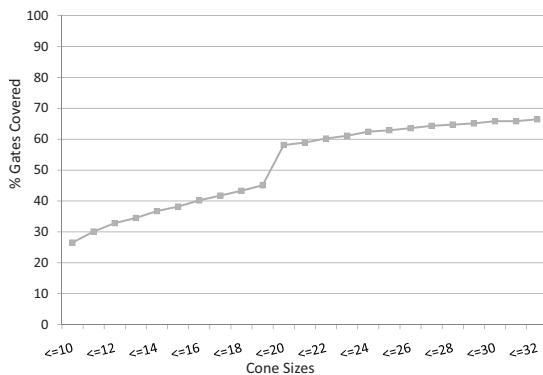
(b) Cones Sizes vs Gates Covered
