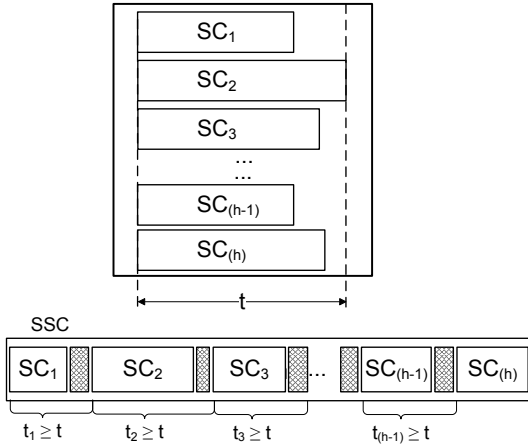
Fig. 3. Mapping of multiple scan chains
