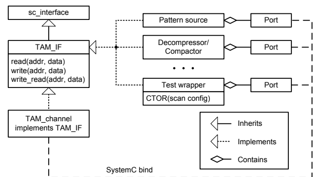
Fig. 2. UML class diagram of test infrastructure entities at transaction level
