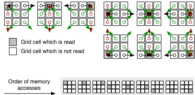
Figure 4: Optimized scheduling of read accesses to particle data.
